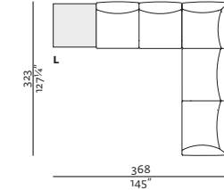
AIRE 90/110 COMPOSITION 05 HIGH ARMREST WITH PLATFORM OR WITH LEGS L/R AIRE 90/110 COMPOSITION 05 LOW ARMREST WITH PLATFORM OR WITH LEGS L/R 368 × 323, height 72 cm 145" × 127¼", height 28¾"
