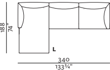
AIRE 110 COMPOSITION 02 LOW ARMREST WITH PLATFORM OR WITH LEGS L/R 340 × 188, height 72 cm 133¾" × 74", height 28¾"
