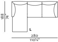
AIRE 90 COMPOSITION 01 LOW ARMREST WITH PLATFORM OR WITH LEGS L/R 280 × 188, height 72 cm 110¼" × 74", height 28¾"
