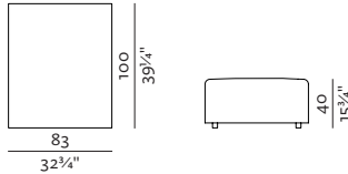
ISLAND 83 83 × 100, height 40 cm 32¼" × 39¼", height 15¾"
