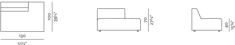
1SEATER EXTENDED 83 (L/R) w 51¼" × d 39¼" × h 28¼" w 130 × d 100 × h 70 cm
