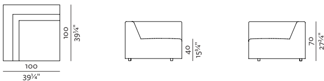
CORNER 100 × 100, height 70 cm 39¼" × 39¼", height 27¾"
