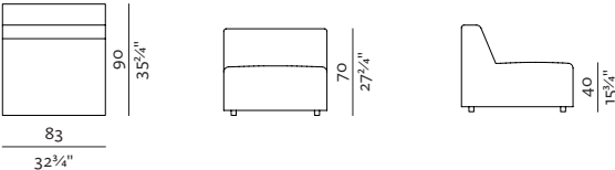
1SEATER 83 83 × 90, height 70 cm 32¾" × 35¾", height 27¾"
