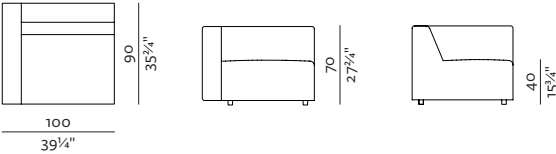
1SEATER + ARMRESTS 83 (L/R) 100 × 90, height 70 cm 39¼" × 35¾", height 27¾"
