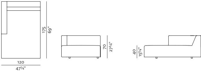
CHAISE LONGUE 175 103 (L/R) 120 × 175, height 70 cm 47¼" × 69", height 27¾"
