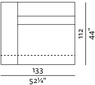
1SEATER WITH ARMRESTS (L/R) 133 × 112, height 70 cm 52¼" × 44", height 27¾"
