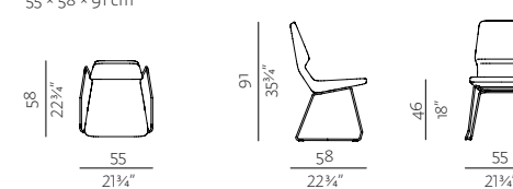
CHAIR SLED BASE WITH ARMRESTS w 22¾" × d 22¾" × h 35¼" 58 × 58 × 91 cm
