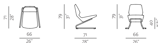
EASY CHAIR CANTILEVER w 26" × d 28" × h 31" 66 × 71 × 79 cm
