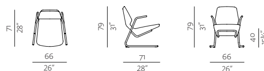
EASY CHAIR CANTILEVER WITH ARMRESTS w 26" × d 28" × h 31" 66 × 71 × 79 cm
