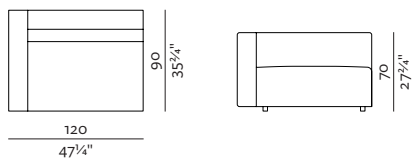
1SEATER + ARMRESTS 103 (L/R) 120 × 90, height 70 cm 47 1 / 4 " × 35 3 / 4 ", height 27 3 / 4 "
