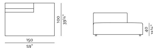
1SEATER EXTENDED 103 (L/R) 150 × 100, height 70 cm 59" × 39 1 / 4 ", height 27 3 / 4 "
