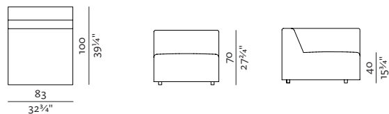
1SEATER 83 83 × 100, height 70 cm 32 3 / 4 " × 39 1 / 4 ", height 27 3 / 4 "
