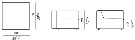
1SEATER + ARMRESTS 83 (L/R) 100 × 100, height 70 cm 39 1 / 4 " × 39 1 / 4 ", height 27 3 / 4 "
