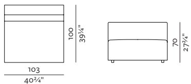
1SEATER 103 103 × 100, height 70 cm 40 3 / 4 " × 39 1 / 4 ", height 27 3 / 4 "
