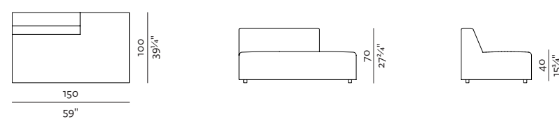
1SEATER EXTENDED 103 (L/R) w 59" × d 39 1 / 4 " × h 28 1 / 4 " w 150 × d 100 × h 70 cm
