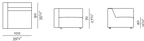
1SEATER + ARMRESTS 83 (L/R) 100 × 90, height 70 cm 39 1 / 4 " × 35 3 / 4 ", height 27 3 / 4 "
