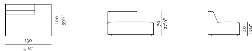
1SEATER EXTENDED 83 (L/R) w 51 1 / 4 " × d 39 1 / 4 " × h 28 1 / 4 " w 130 × d 100 × h 70 cm
